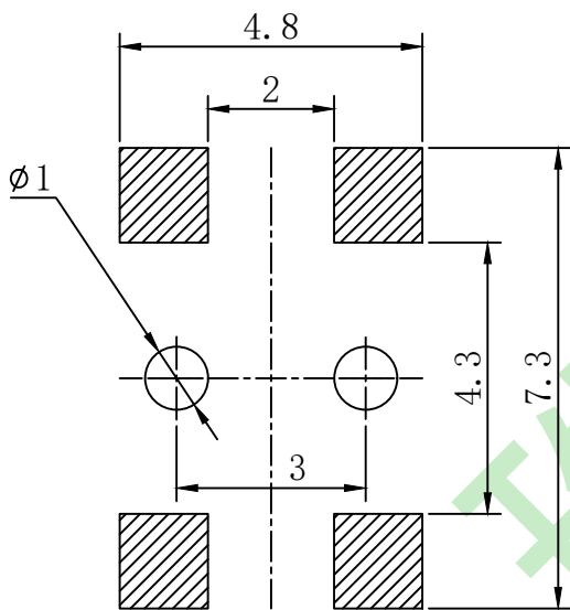
PCB焊接图 PCB. WELDING DRAWING
